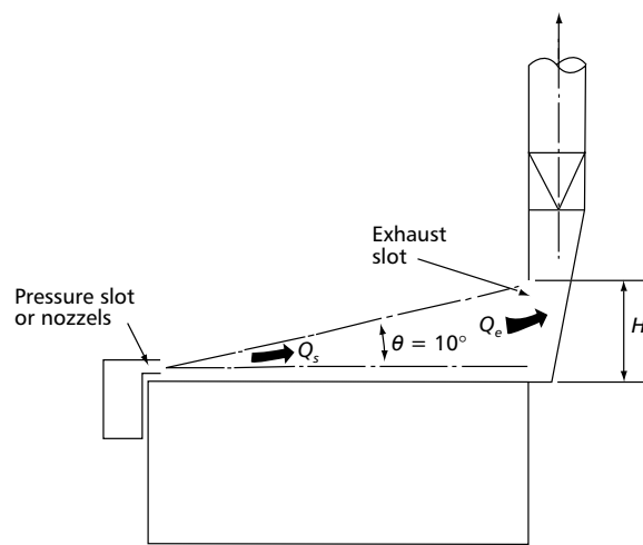
Figure 2.40 Push-pull hood
