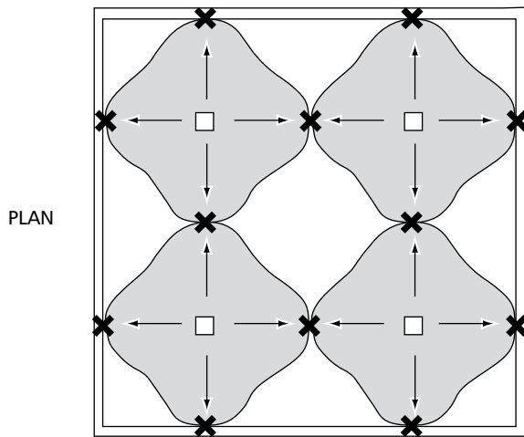
(a) Four-way ceiling diffusers, symmetrical layout
