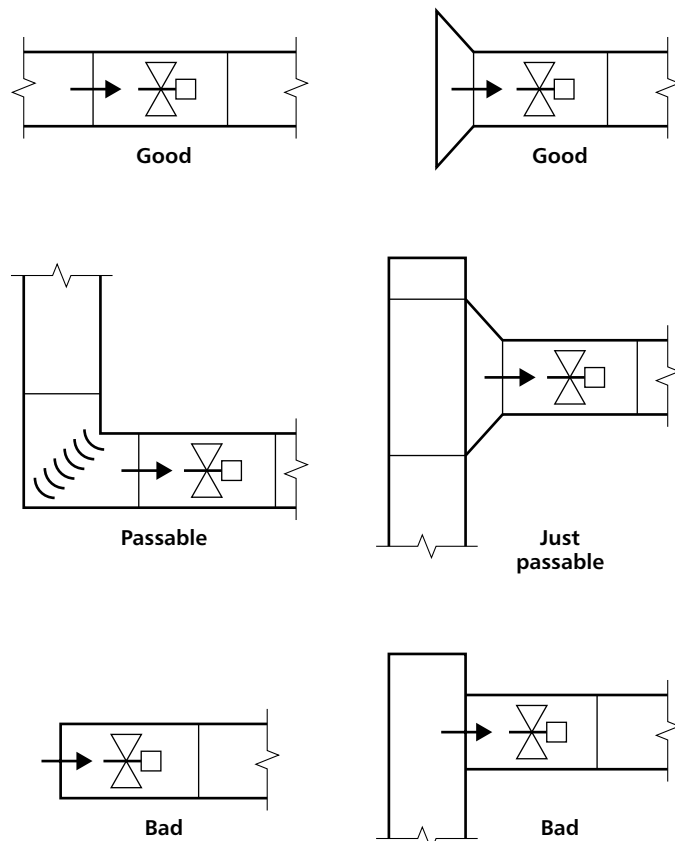
Figure 2.50 Axial fans; inlet connections
