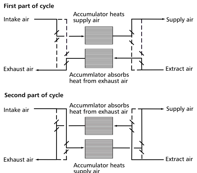
Figure 2.23 Regenerator
