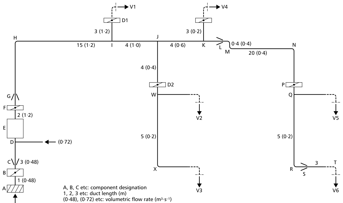
Figure 2.A5.1 Duct layout with lengths (m) and flow rates ( \text{m}^3\text{s}^{-1} )
